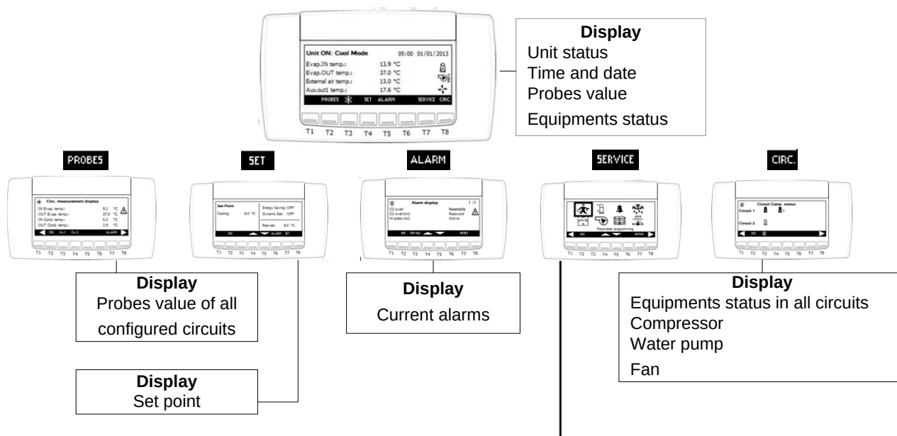
Main screen
