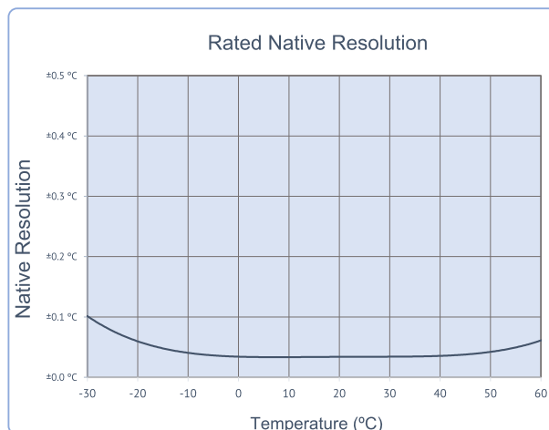
Figure 7: Rated Temperature Resolution Chart
